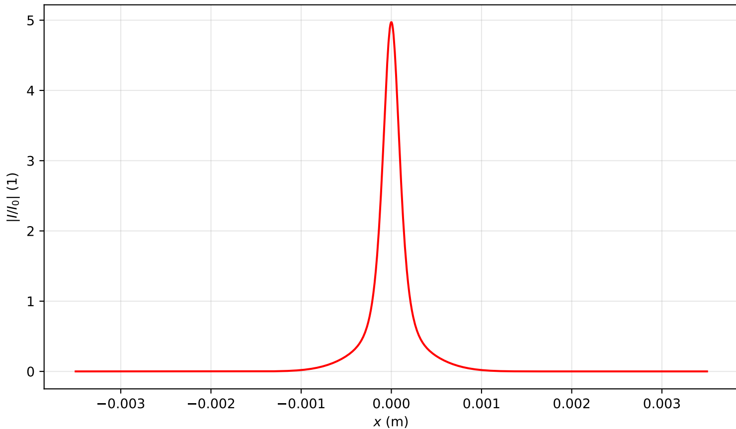
Intensity profile I(x, y = 0, z = 0.716)/I_0 , P_{in}=2.5P_{cr} , artificial time
